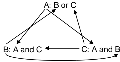
Figure 5: Random Boolean Network (RBN) Example. The state of the network is given by the boolean values of A , B , and C . At each timestep, the state values are updated based on their values in the previous timestep. In the approach of Dellaert and Beer (1996), the current state of a cell is given by the current state of its RBN. Individual bits in the state signal events like cell splitting or creating connections between cells. RBNs were introduced by Kauffman (1993) to simulate the protein expression patterns in cells in a developing embryo. RBNs are computationally less expensive than full-blown GRN implementations (figure 4), while exhibiting similar dynamics.
