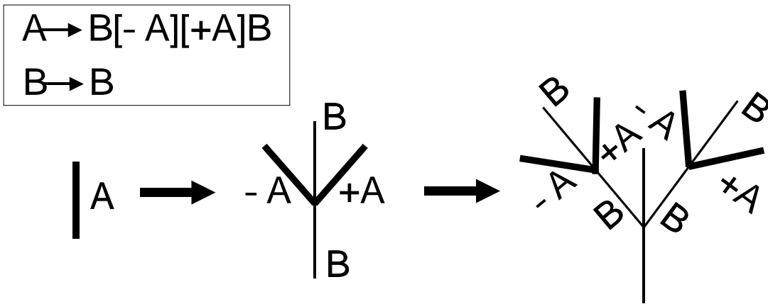
Figure 1: Grammatical Approach Example (L-systems; Lindenmeyer 1968).. The two rewrite rules (inset) describe the growth of a tree-like morphology. The symbol A , shown as a thick line in the tree, is the only symbol that is rewritten in this grammar. The symbol B , which does not expand, becomes a thin branch, and - and + determine relative angles of branches expanded from A symbols. This example illustrates how a few simple generative rules can encode a large structure with many components.
